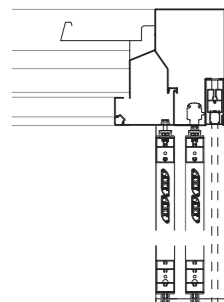
Multilayer screen system Chiusure multiple
